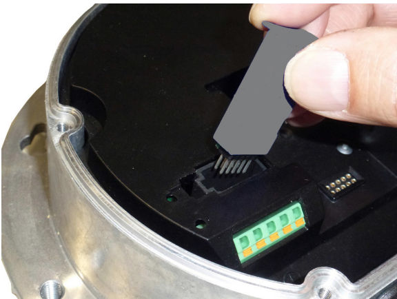
Example for mounting the bluetooth stick
